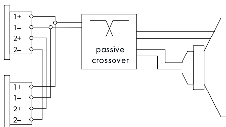
Connector wiring
